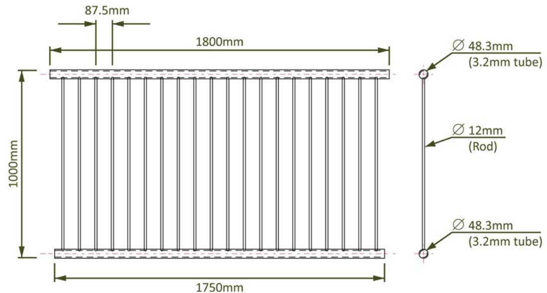
1800mm wide Pedestrian Panel
