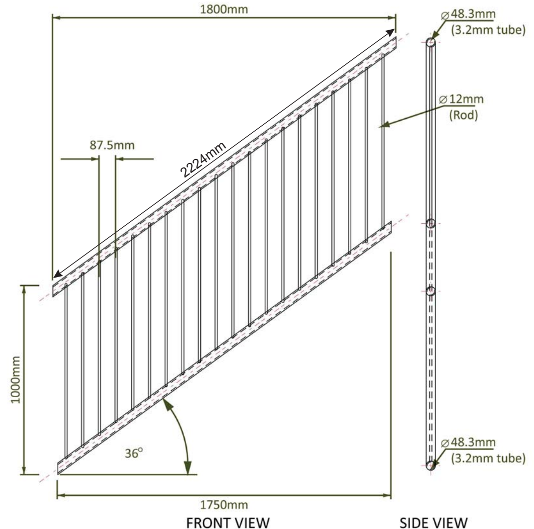
1800mm wide Pedestrian Panel - other angles available on special order
